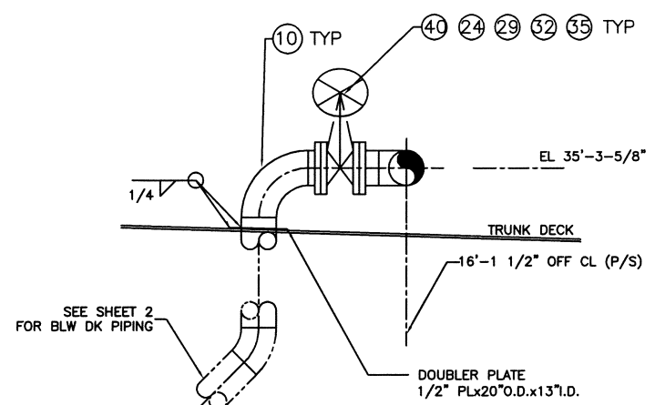
SECTION 31-D STDB SIDE SHOWN LOOKING FWD PORT SIMILAR BUT OPPOSITE HAND SCALE: 3/8" = 1'-0"
