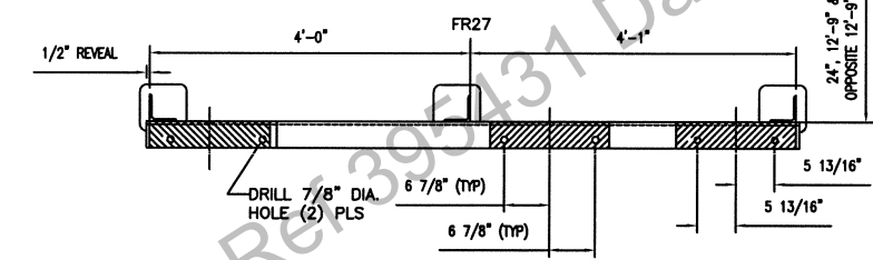
SECTION 28-C FIELD CHECK U-BOLT SIZE BEFORE DRILLING HOLES TYP. SCALE: 3/4" = 1'-0"
