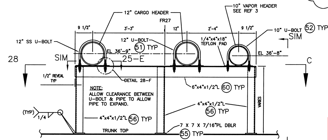
SECTION 28-A PIPE SUPPORT AT TRANSV. HEADERS STBD LOOKING INBD PORT OPPOSITE SCALE: 3/4" = 1'-0"
