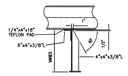
SECTION 27-E 12" PIPE SHOWN / 10" SIMILAR SCALE: 3/4" = 1'-0"
