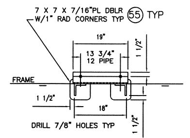
SECTION 25-E 12" PIPE SHOWN FOR 10" PIPE ONLY U-BOLT SIZE CHANGE FIELD CHECK U-BOLT SIZE BEFORE DRILLING HOLES TYP. SCALE: 3/4" = 1'-0"
