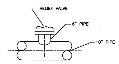
DETAIL 32-A SECTION OF RELIEF VALVE SCALE: 3/4" = 1'-0"
