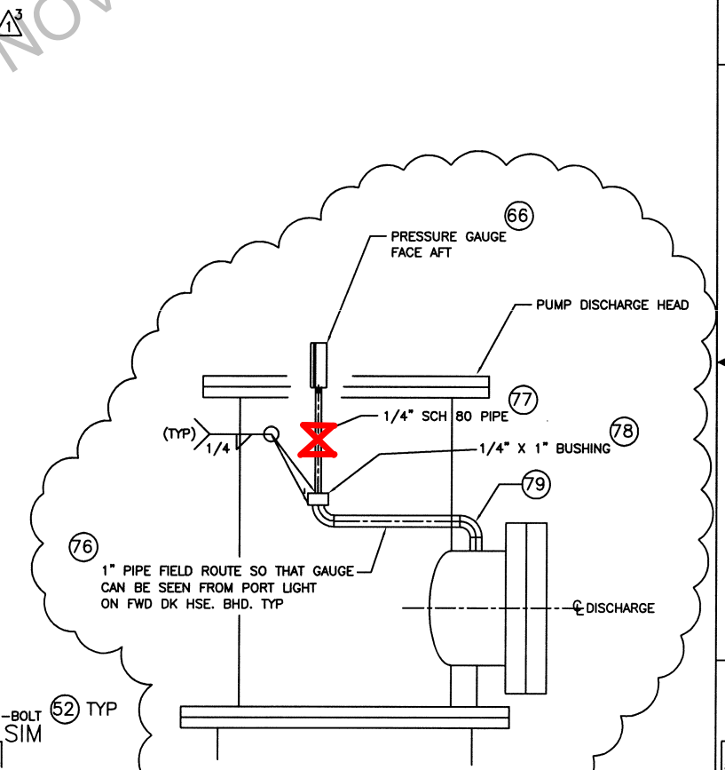
DETAIL 26-B GAUGE DETAIL SCALE: 1 1/2" = 1'-0"
