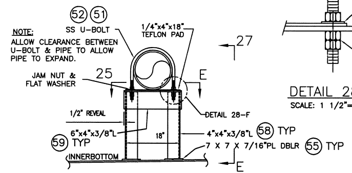
SECTION 29-E 12" PIPE SHOWN / 10" SIMILAR SCALE: 3/4" = 1'-0"
