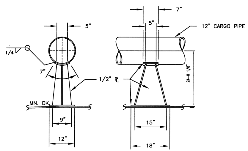
DETAIL 31-B PIPE ANCHOR ABOVE DECK SCALE: NTS
