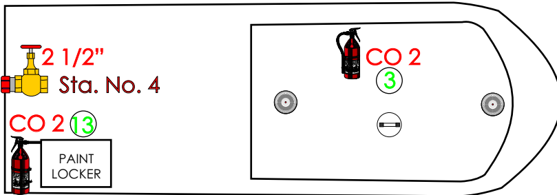
Boat Deck
