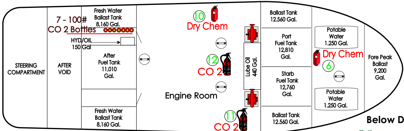
Main Deck
