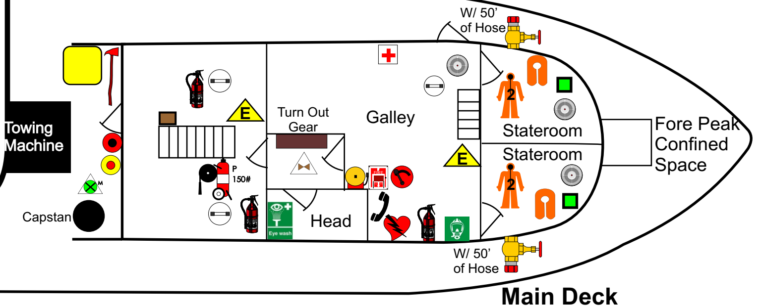
02 Deck
