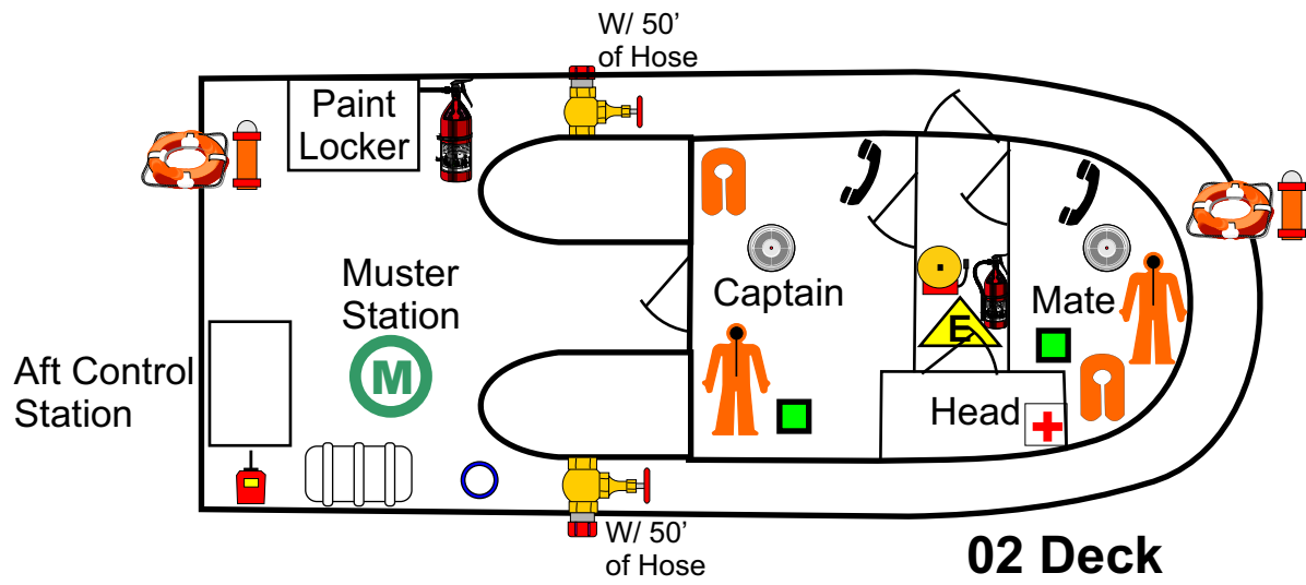
Pilothouse
