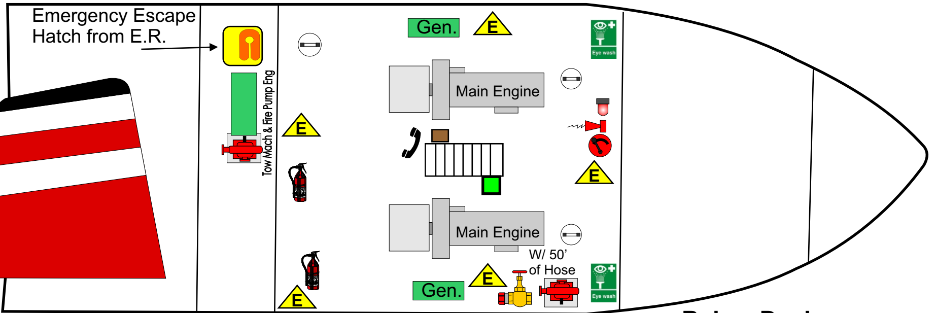
Below Deck
